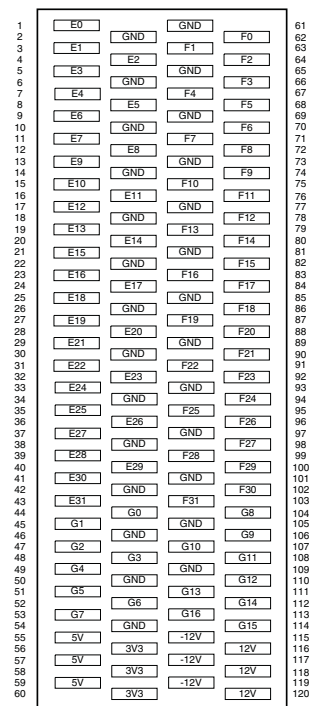
Figure A-2 HDRB socket pin numbering
